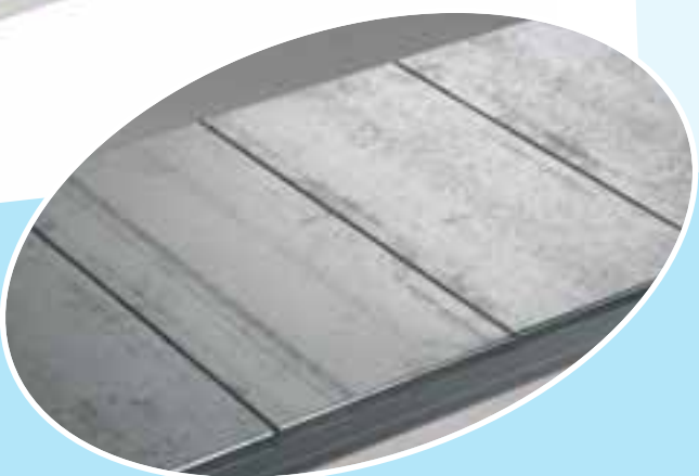
Galvanised Steel Shelf Panels Span box beams to form a steel shelf. Panels 300/374/600mm wide.
